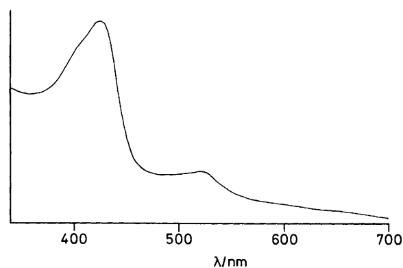
FIGURE 6 Absorption spectrum of the \mu -oxo-dimer of [Mn^{IV}(tpp)] formed by reaction of [Mn^{III}(tpp)] with iodossylbenzene in CH_2Cl_2 solution
