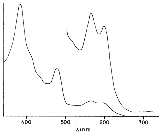
FIGURE 5 Absorption spectrum of the \pi -radical cation of [Mn^{III}(tpp)] formed by reaction of [Mn^{III}(tpp)] with phenoxathiinium hexachloroantimonate in CH_2Cl_2 solution
