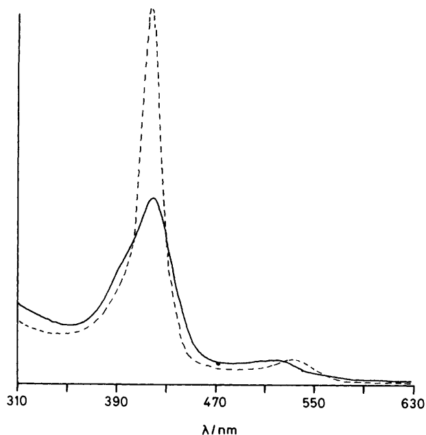
FIGURE 4 Absorption spectra of [Mn^{IV}(tpp)] (—) and [Mn^{V}(tpp)] (---) in ctac micelles at pH 12 formed by reaction with bromate and hypochlorite respectively
